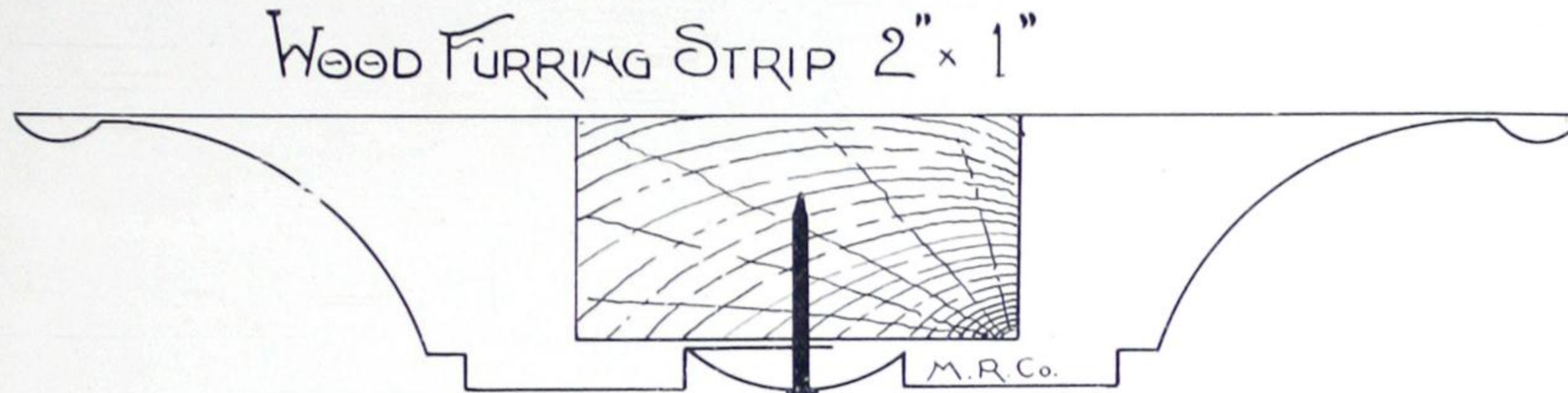
Fig. 3400.—Section of Joint on Plates Nos. 400, 401, 402, 403, and 479.
